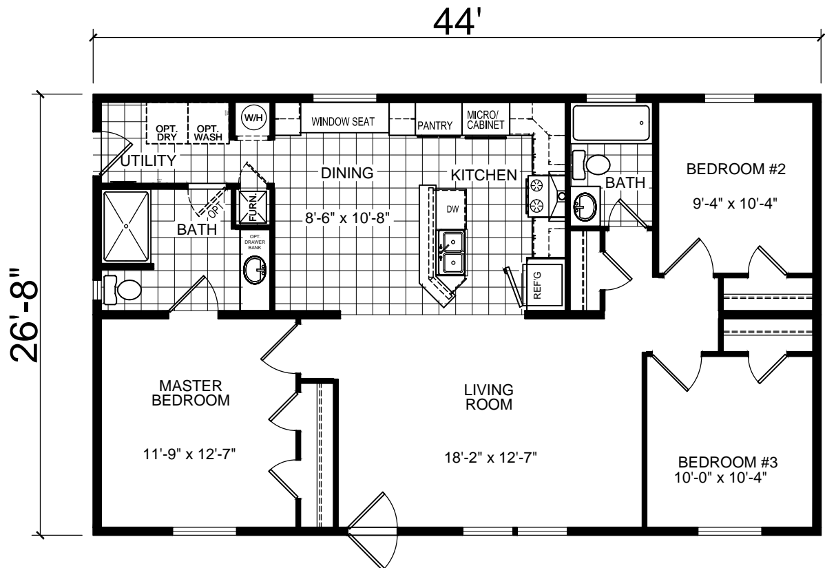
MODEL A-24402 3 BEDROOM, 2 BATH NOMINAL SIZE: 28' x 48' ACTUAL SIZE: 26'-8" x 44'-0" TOTAL AREA: 1173 SQ. FT.
